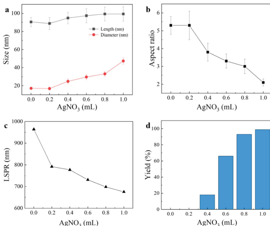
Fig. 5 The size, aspect ratio, LSPR and yield of asymmetric nanostructures with different amount of 4.0 mM \text{AgNO}_3 (0.2–1.0 mL). (a) The size of final products with different amount of \text{AgNO}_3 . Especially, 0 mL of \text{AgNO}_3 corresponds to the sample AuNR-Pt. With the increase of \text{AgNO}_3 amount, the particles become bigger and the diameter increased faster than the length. (b) The aspect ratio of different products. With the increase of \text{AgNO}_3 , the aspect ratio decreased. (c) The position of LSPR in different (AuNR-Pt)-Ag. As the amount of \text{AgNO}_3 increased, the position of the LSPR gradually blue-shifted. (d) The yield of asymmetric (AuNR-Pt)-Ag. The core-shell structures cannot be observed with 0.2 mL \text{AgNO}_3 . Especially, when the amount of \text{AgNO}_3 is 1.0 mL, the yield of asymmetric nanostructures can reach >99%.
