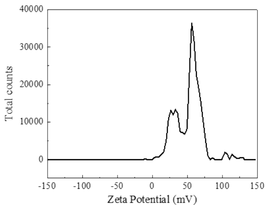
Figure S2. The DLS image of the tri-metallic (AuNR-Pt)-Ag nanostructure in 1.0 mL AgNO 3 , the zeta-potential image of asymmetric (AuNR-Pt)-Ag nanostructure. The potential is greater than +30 mV, so this nanosystem is very stable.
