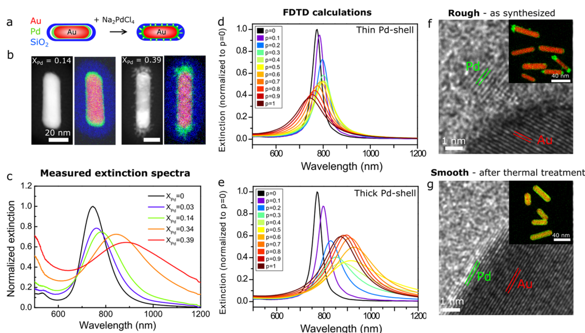
Figure 3. Control over the Pd shell morphology: switching between smooth and rough Pd layers to alter the plasmonic properties. (a) Schematic representation of the Pd overgrowth with increasing Na 2 PdCl 4 concentration, leading to an increase in roughness of the Pd shell. (b) HAADF-STEM images and corresponding EDX intensity maps of Au@Pd@SiO 2 NRs grown with 0.18 mM (X Pd = 0.14) and 0.83 mM (X Pd = 0.39). (c) Measured extinction spectra of the Au@Pd@SiO 2 NRs in water, grown with 0–0.83 mM Na 2 PdCl 4 and X Pd = 0–0.39. (d, e) Finite-difference time-domain (FDTD)-calculated extinction spectra of Au@Pd@SiO 2 NRs with a thin (d) and a thick (e) Pd shell as a function of the Pd packing fraction p of the shell, where p < 1 and p = 1 correspond to a discontinuous and continuous Pd shell, respectively (see the Experimental Section for details). The Au@Pd@SiO 2 NRs with a thin and a thick Pd shell correspond to experimental results with 0.083 mM Na 2 PdCl 4 (Au core: 58.5 × 17.7 nm; Au@Pd NR: 60.5 × 19.7 nm) and 0.83 mM Na 2 PdCl 4 (Au@Pd NR: 78.6 × 19.4 nm), respectively. (f, g) HRTEM image and EDX intensity map of Au@Pd@SiO 2 NRs with a rough shell morphology before (f) and after (g) thermal treatment for 1 h at 300 °C in H 2 . See Table S3 for the full set of experimental details.
